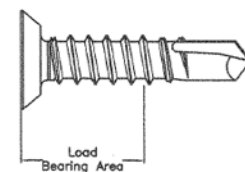
FIGURE 2—TEKS SELECT UNDERCUT PHILLIPS FLAT HEAD (UPFH) FASTENER
