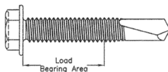
FIGURE 1—TEKS SELECT HEX WASHER HEAD (HWH) FASTENER
