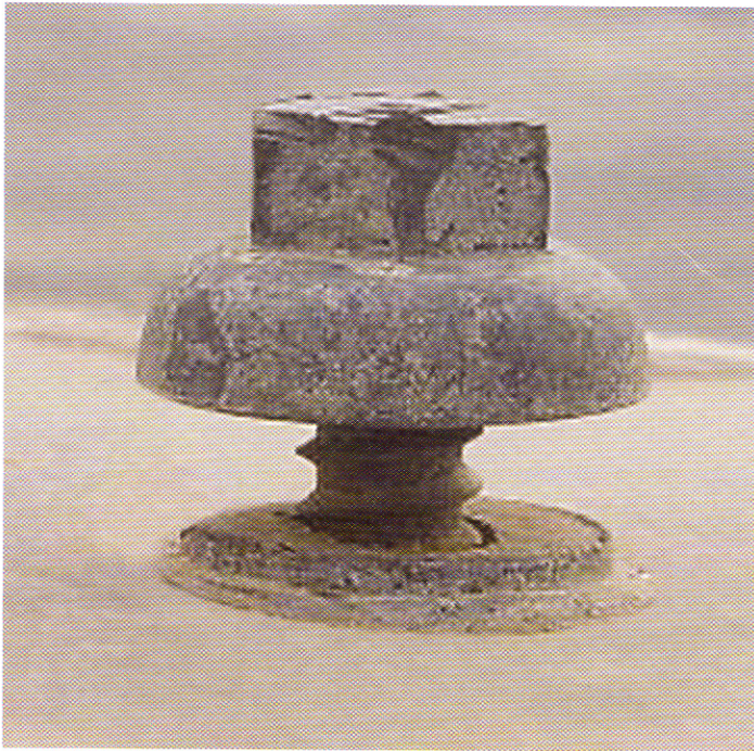
The Itasca, Ill.-based ITW Buildex Anti Back Out self-drilling screw resisted back out during all testing. The company added a patent-pending thread feature that prevents back out caused by thermal movement, keeping roof systems tightly sealed.
