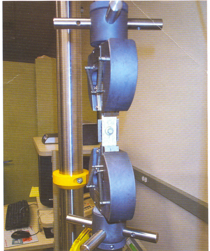
This apparatus applied tension and compressive forces to simulate the expansion and contraction movements of metal roof panels during 12 years of thermal cycles.
